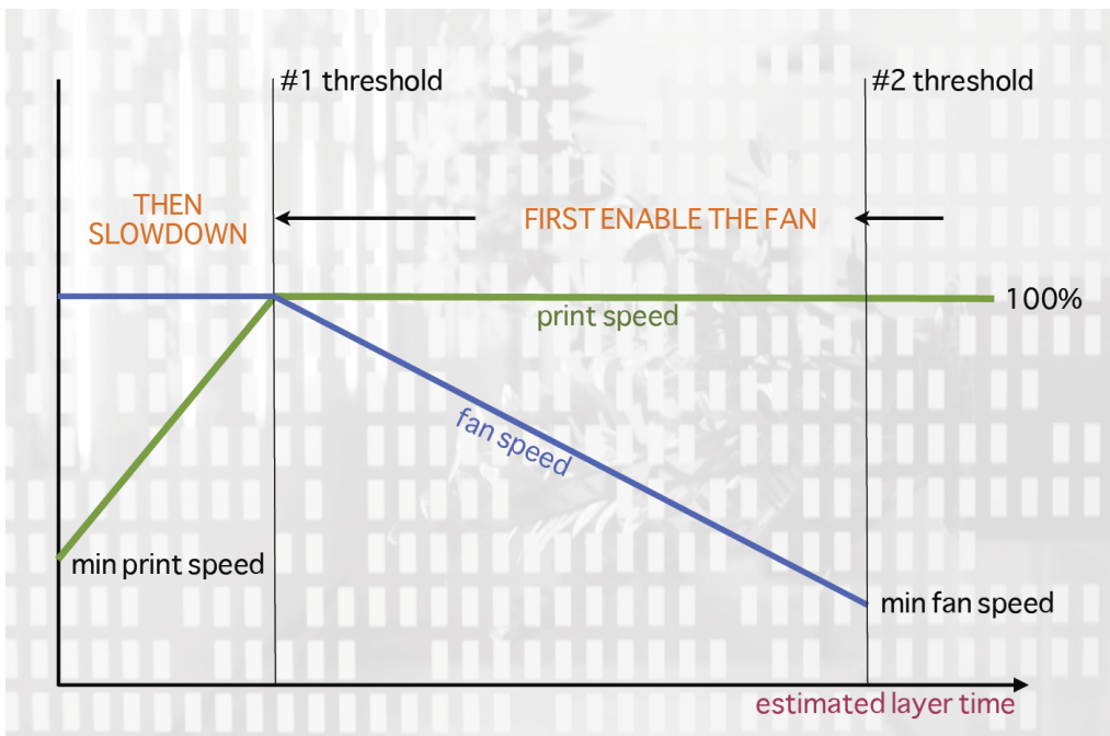
Figure 5.35: Cooling strategy.
