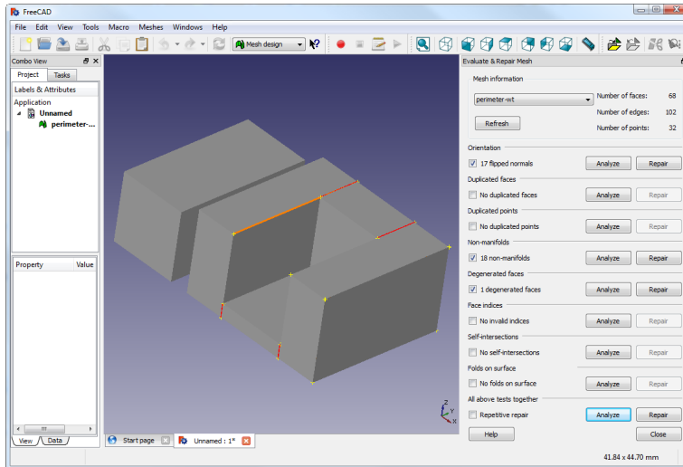
Figure 5.58: FreeCAD part repair.
