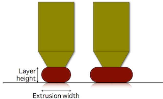
Figure 2.64: Extrusion Width.
